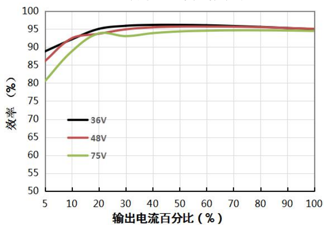
VCF4828QBO-400W(F/H)R3(-N)
