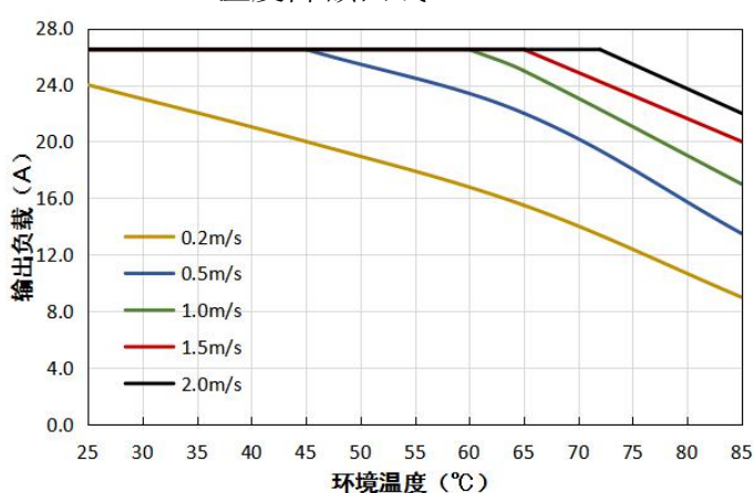
VCF4815QBO-400WHR3(-N) 温度降额曲线 (Vin=48V)
