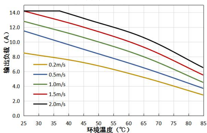
VCF4828QBO-400WR3(-N) 温度降额曲线 (Vin=48V)
