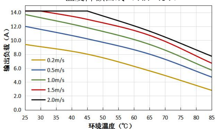
VCF4828QBO-400WFR3(-N)
