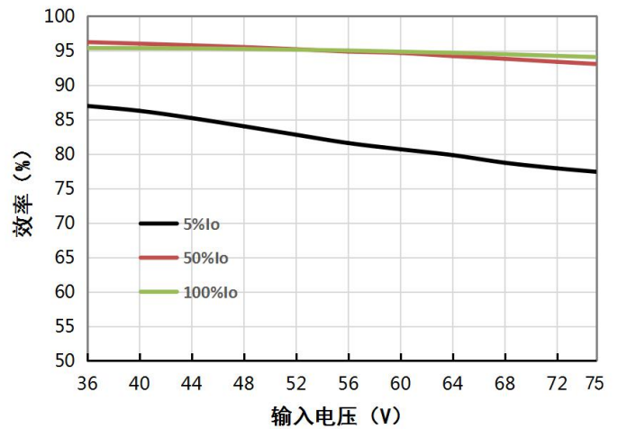
VCF4824QBO-400W(F/H)R3(-N)
