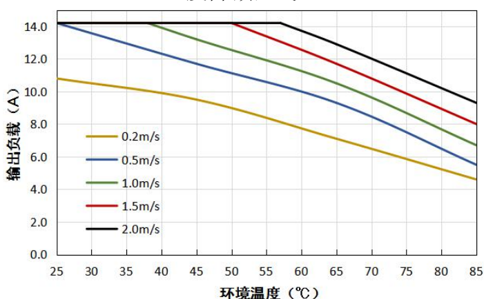
VCF4815QBO-400WFR3(-N)
