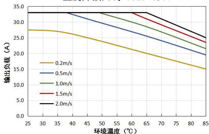
VCF4812QBO-400WHR3(-N) 温度降额曲线 (Vin=48V)
