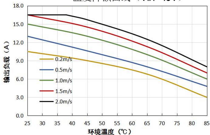
VCF4824QBO-400WR3(-N) 温度降额曲线 (Vin=48V)
