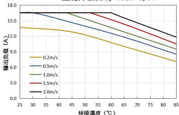
VCF4812QBO-400WFR3(-N)
