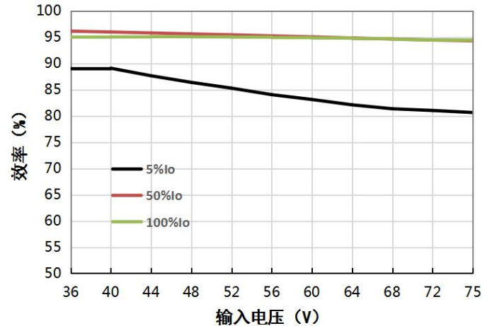
VCF4828QBO-400W(F/H)R3(-N)
