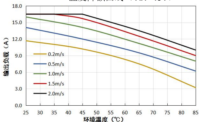
VCF4824QBO-400WFR3(-N)
