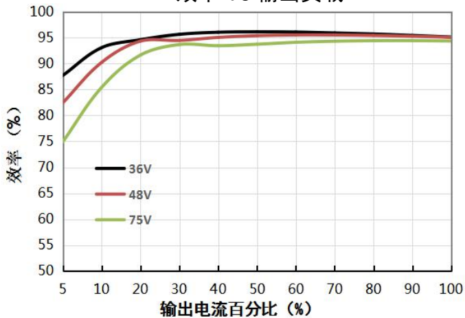
VCF4828QBO-400W(F/H)R3(-N)
