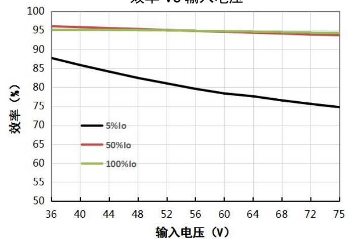
VCF4828QBO-400W(F/H)R3(-N)
