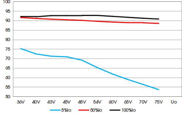
VCF4812EBO-50W(F)R3-N 效率VS输入电压
