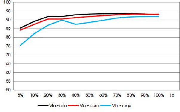
VCF4812EBO-50W(F)R3-N 效率VS输出负载
