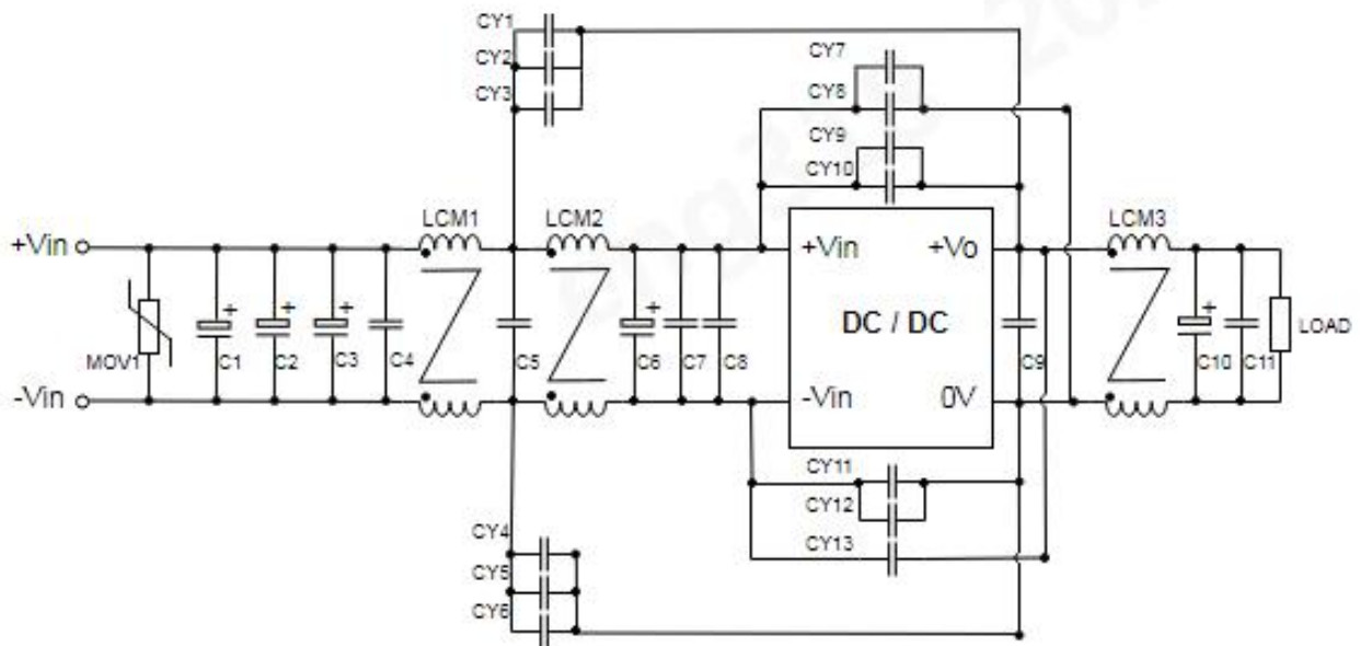
VCF4828/48EBO-100W(F)R3-N
