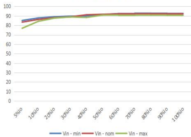
VCF2412EBO-120W(F)R3-N 效率VS输出负载
