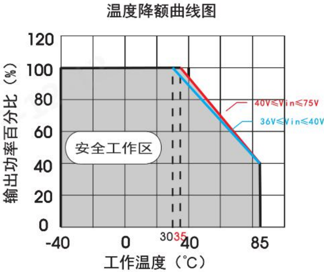
VCB4805SBO-40WR3(-N)
