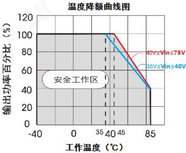
VCB4812SBO-40WR3(-N)
