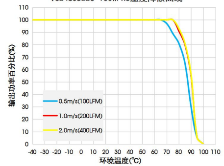
VCB4805EBO-100WR3温度降额曲线
