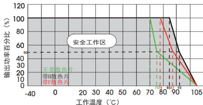
UWTH1D24/28/48/54LD-20W(H/F)R3 温度降额曲线 (Vin=110V, 无风)
