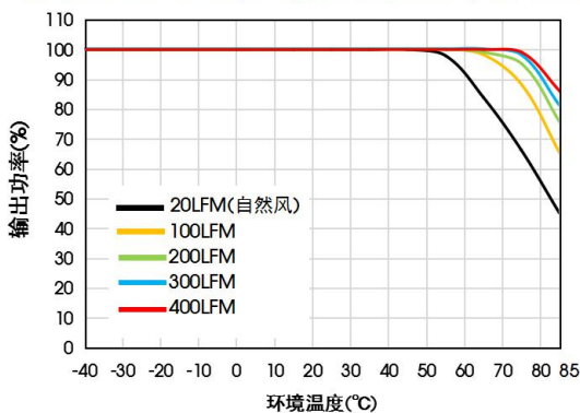
URF4824QB-100WR3 温度降额曲线 (Vin=24V)
