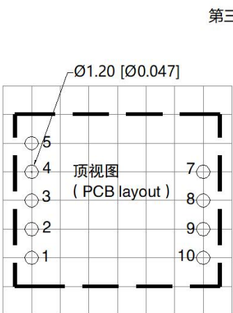
注：栅格距离 2.54*2.54mm
