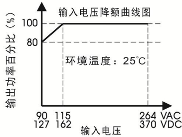
LOF750-20Bxx 输入电压降额
