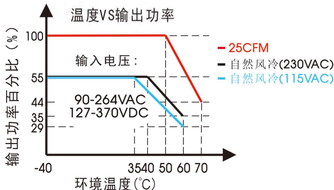
LOF450-20B24/27/36/48/54-CF (满载 450W 带 25CFM 风扇)
