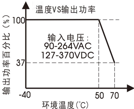
LOF450-20B12/15/18/19-CF (满载 400W 带 25CFM 风扇)
