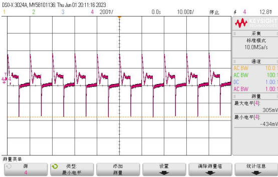
V_{in}=115VAC 10%-100%动态
