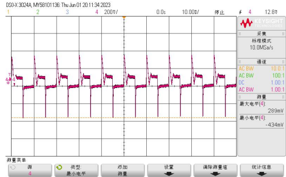
V_{in}=230VAC 10%-100%动态
