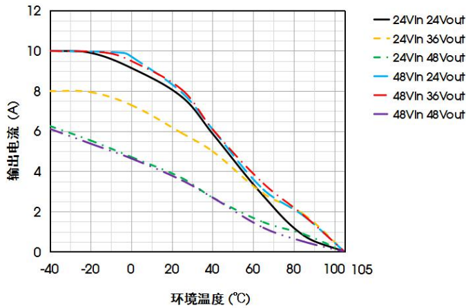
KUB4836EB-10A (-RS) 温度降额曲线 (20LFM)
