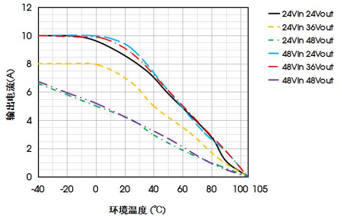
KUB4836EBF-10A (-RS) 温度降额曲线 (20LFM)
